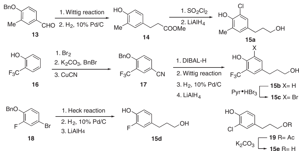
Scheme 2. Synthesis of 15a–15e .
