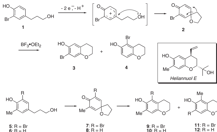
Scheme 1. Synthesis of the spirodienones, and its conversion into the chroman derivatives.
